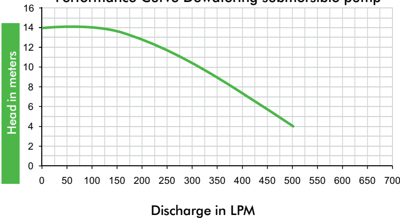
Performance Curve Dewatering submersible pump
